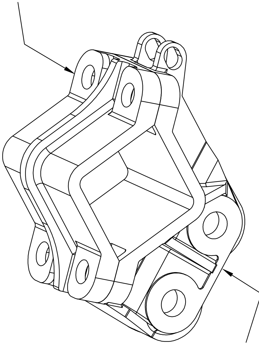
KAG 012 - Shank Carrier
